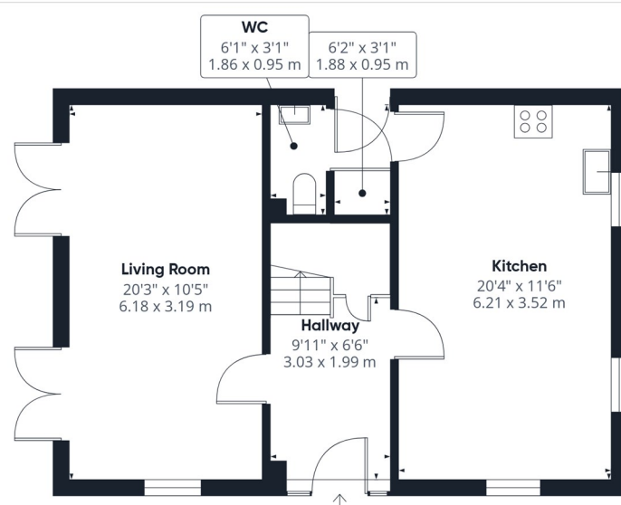
Floor 0 Building 1
