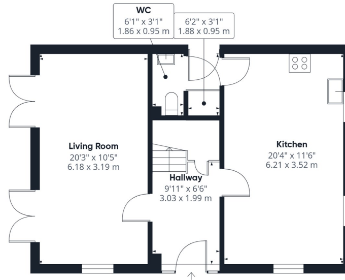
Floor 0 Building 1
